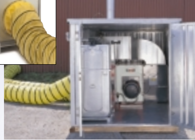
Mobile heating plants HM 200 The solid heating plant for building sites, tents, halls. Rated heating power 173 kW
